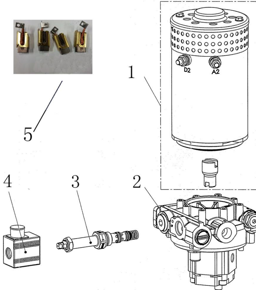
Fig.27 Pump,24V3.2KW4.0cc(HPI)
