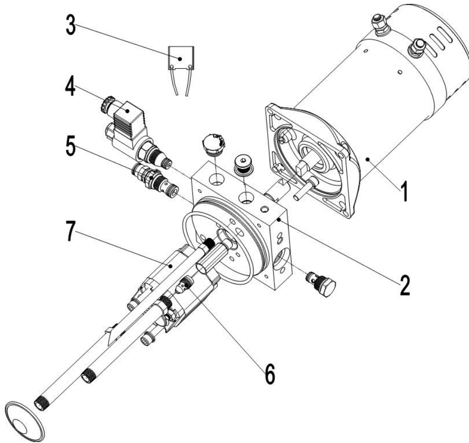
Fig.28 Pump,24V3.0KW3.3cc(VIBO)
