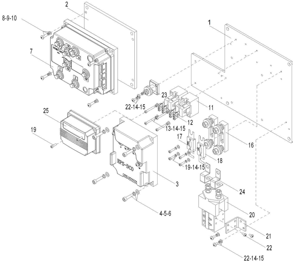
Fig.31 Electrical control components
